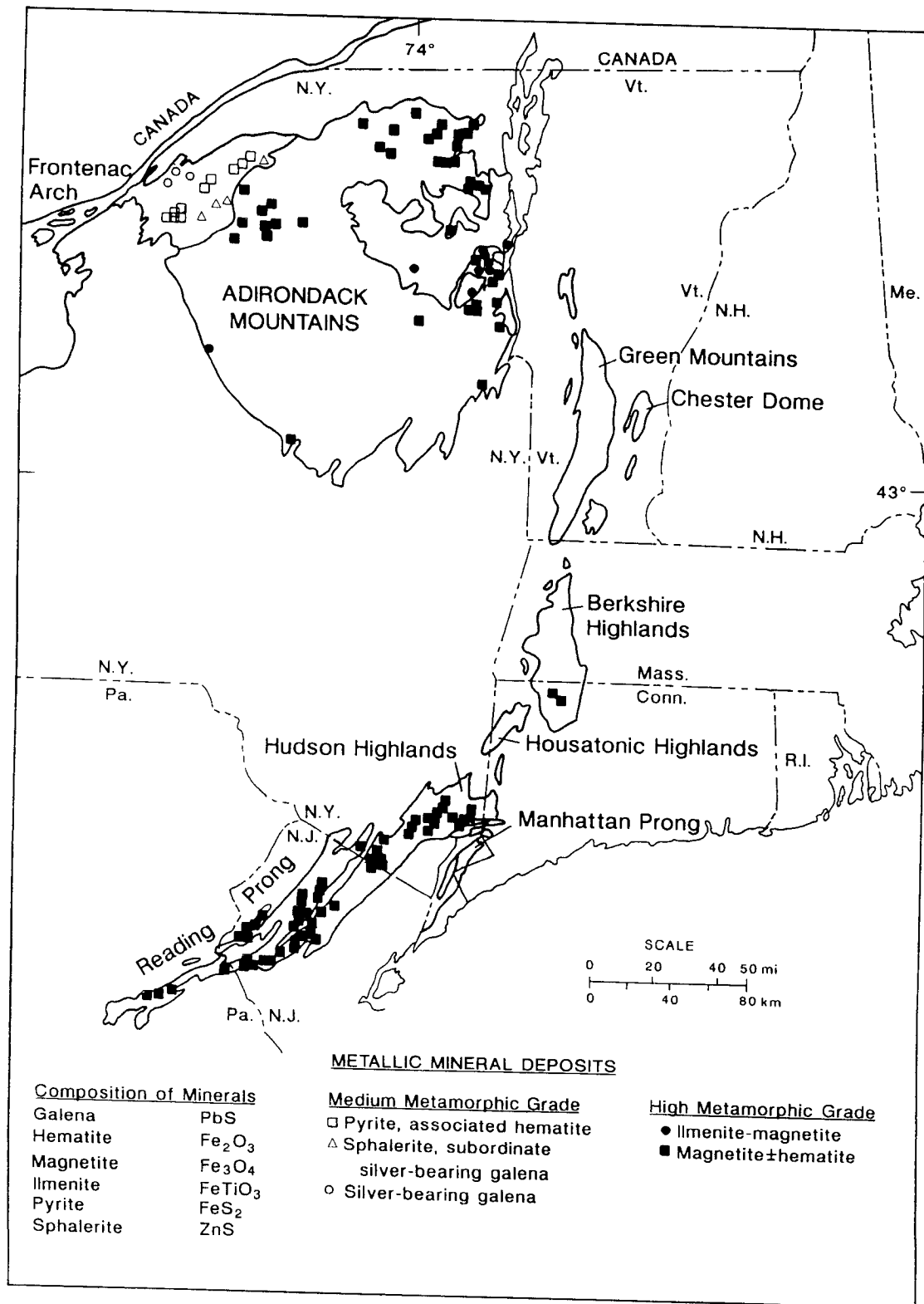
Figure 15.2. Metal deposits in Proterozoic rocks of the northeastern United States.
